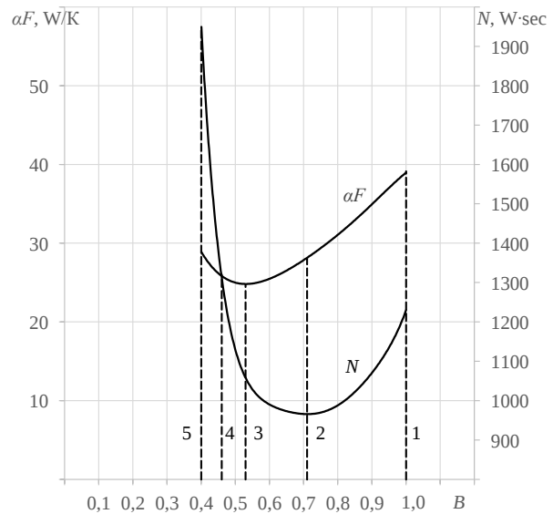
Fig. 8. Dependence of the N , \alpha F values of the TPP complex with their serial electrical connection on the relative operating current B at T_c=300\text{K} ; \Delta T=40\text{K} ; l/S=4.5 :
