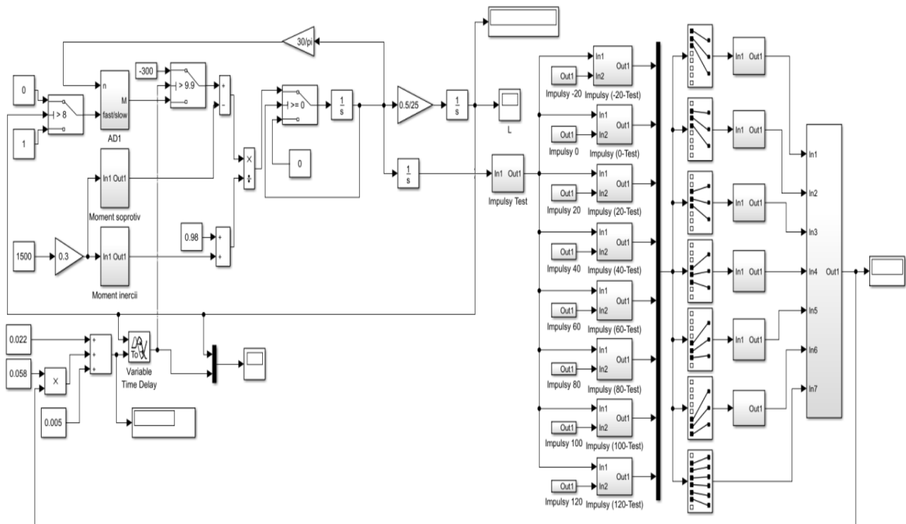
Fig. 2. Simulation model of an elevator installation with a control system in the Matlab / Simulink environment
