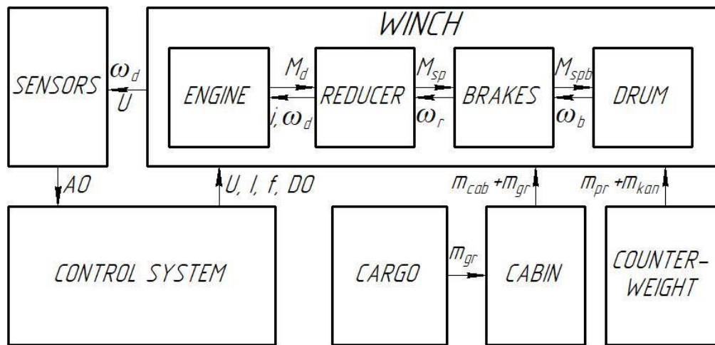
Fig. 1. Block diagram of the elevator installation
