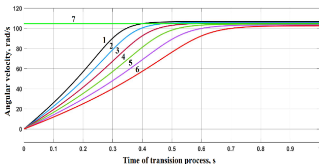
Fig. 3. Transients during engine start
