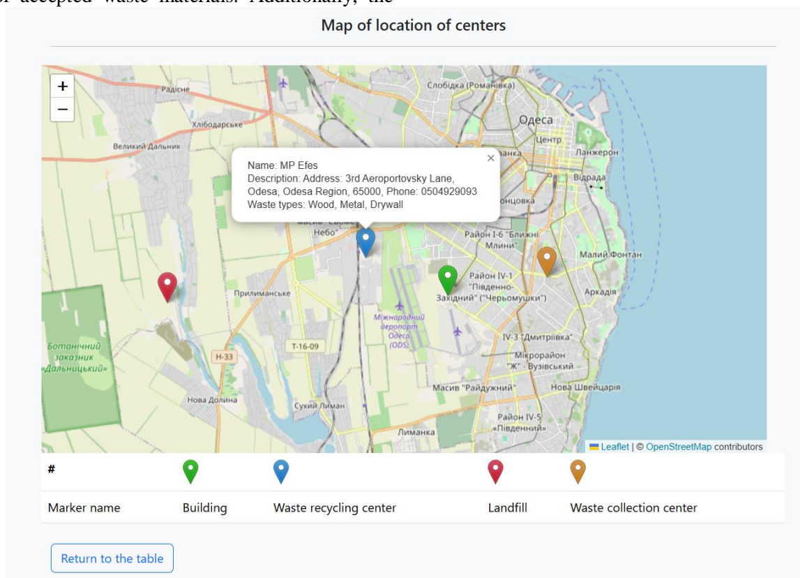
Fig. 6. The screen form for the geospatial data about waste collection points closest to the waste generation site
