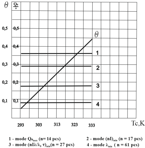
Fig. 5. Dependence of the relative temperature drop \Theta and cooling capacity per thermocouple Q_0/n on the medium temperature T_c for different initial characteristic current operating conditions at T_c = 338\text{K} at I/S = 293; K, = 4.5;
