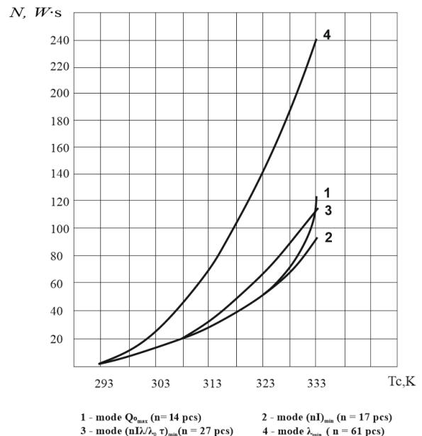
Fig. 7. Dependence of amount of energy N expended on medium temperature T_c for different initial characteristic current modes at
