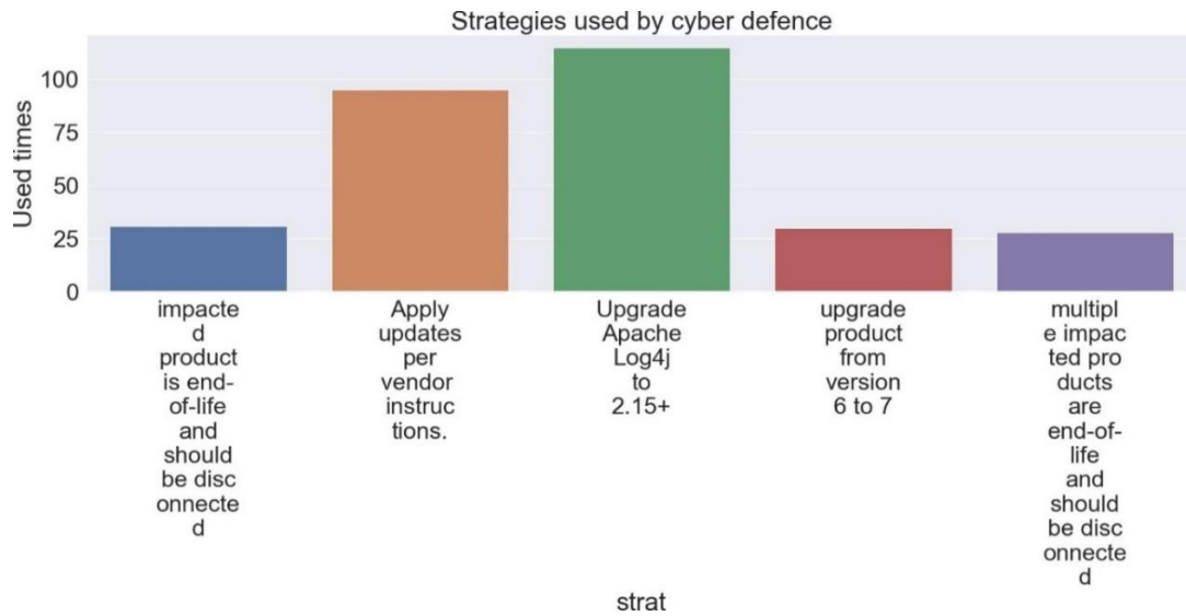
Fig. 5. Strategies used by cyber defence based on the 300 draws of the game with CISA dataset Source: compiled by the authors
