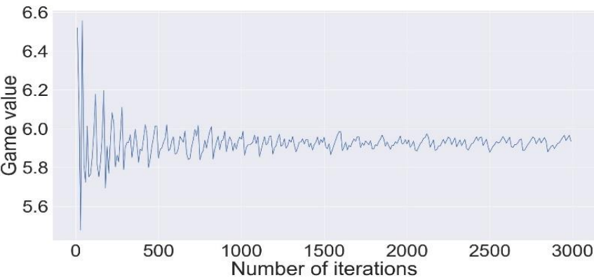
Fig. 3. The convergence of Brown-Robinson algorithm, showing mean value of the game V depending on number of iterations with the use of CISA dataset Source: compiled by the authors
