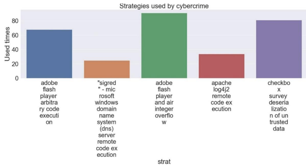
Fig. 4. Strategies used by cybercrime based on the 300 draws of the game with CISA dataset Source: compiled by the authors
