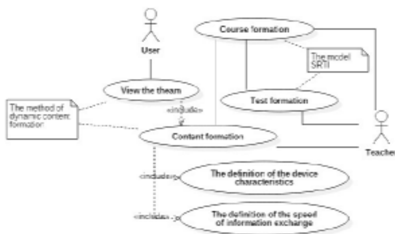
Fig. 3. Diagram of use cases of the information system SDDC of the dynamic formation content in real-time
