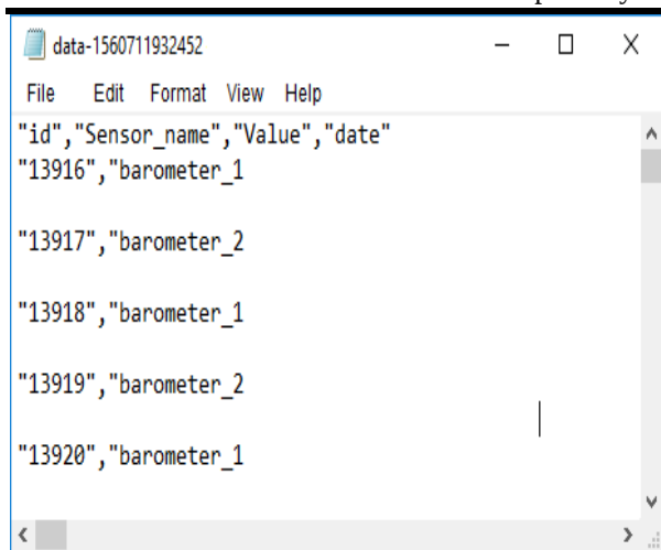
Fig. 3. Data representation in a non-relational database
