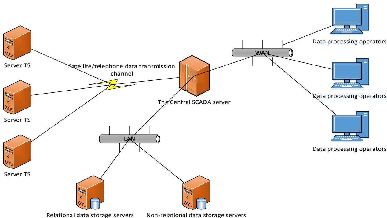
Fig. 4. Network architecture of SCADA-system scheme using multi-structure data storage
