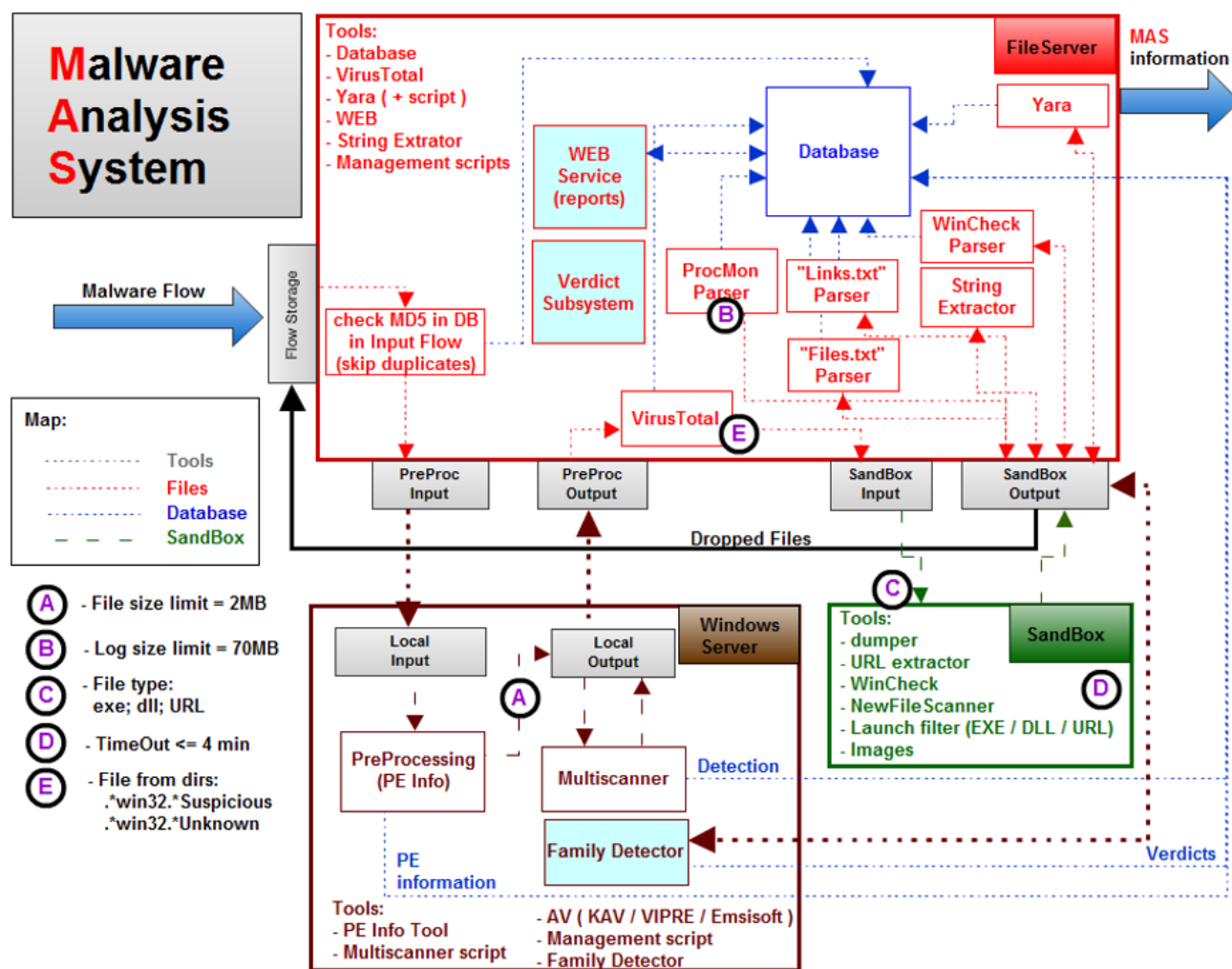
Fig. 3. The main components of the MAS cloud service
