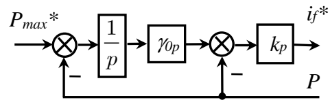
Fig. 10. Maximum HESG power controller diagram of type 101
