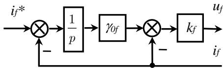
Fig. 8. Field excitation current controller of generator of type 101
